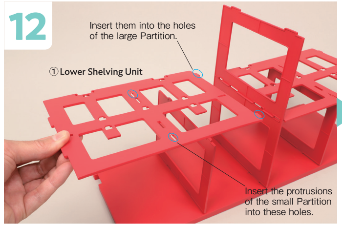
Assemble the ① Lower Shelving Unit above the Partition on the left by fitting its holes and protrusions to the large and small Partitions.
