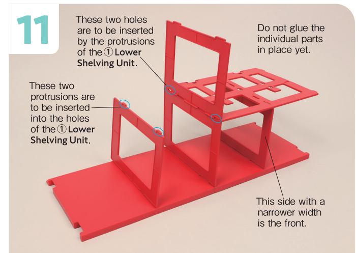
Now check how the Shelving is assembled. First, assemble the large and small Partitions and the Shelving from issue 59 to the Base Plates.
