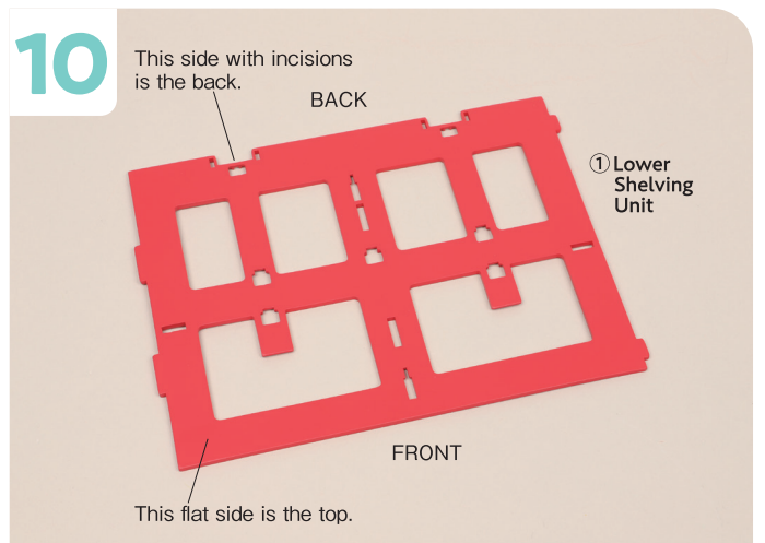
Check the orientation of the ① Lower Shelving Unit.
